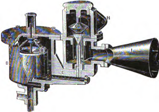
FIG. 315. —The "Phenix" Daimler Carburetter. A is the gasoline needle valve; B, the weighted controlling levers; C, the float; D, the float chamber; E, the gasoline supply tube; F, the spraying nozzle; G, the "mushroom" spray deflector; H, the port leading to the cylinder chamber; I, the air inlet. The air entering the mixing chamber follows the course of the arrows.
